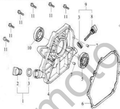
E-2 曲轴箱盖组件 CRANKCASE COVER ASSY
