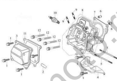
E-3 气缸头 气缸头盖总成 CYLINDER HEAD &amp; CYLINDER HEAD COVER ASSY
