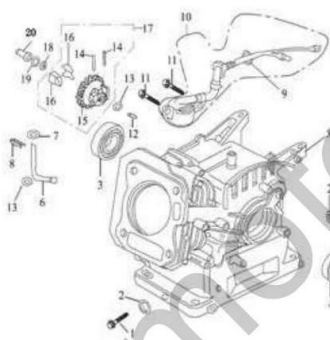
E-1 曲轴箱组合 CRANKCASE ASSY
